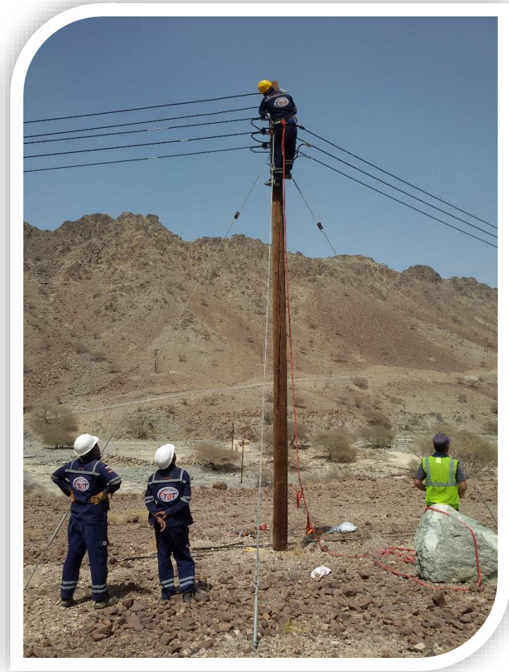
Work in progress on LV and 11kV Overhead Lines
